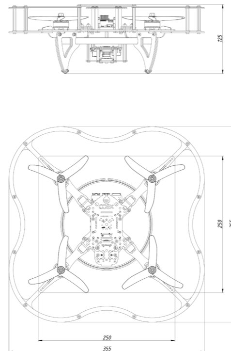
Dimensional drawing
